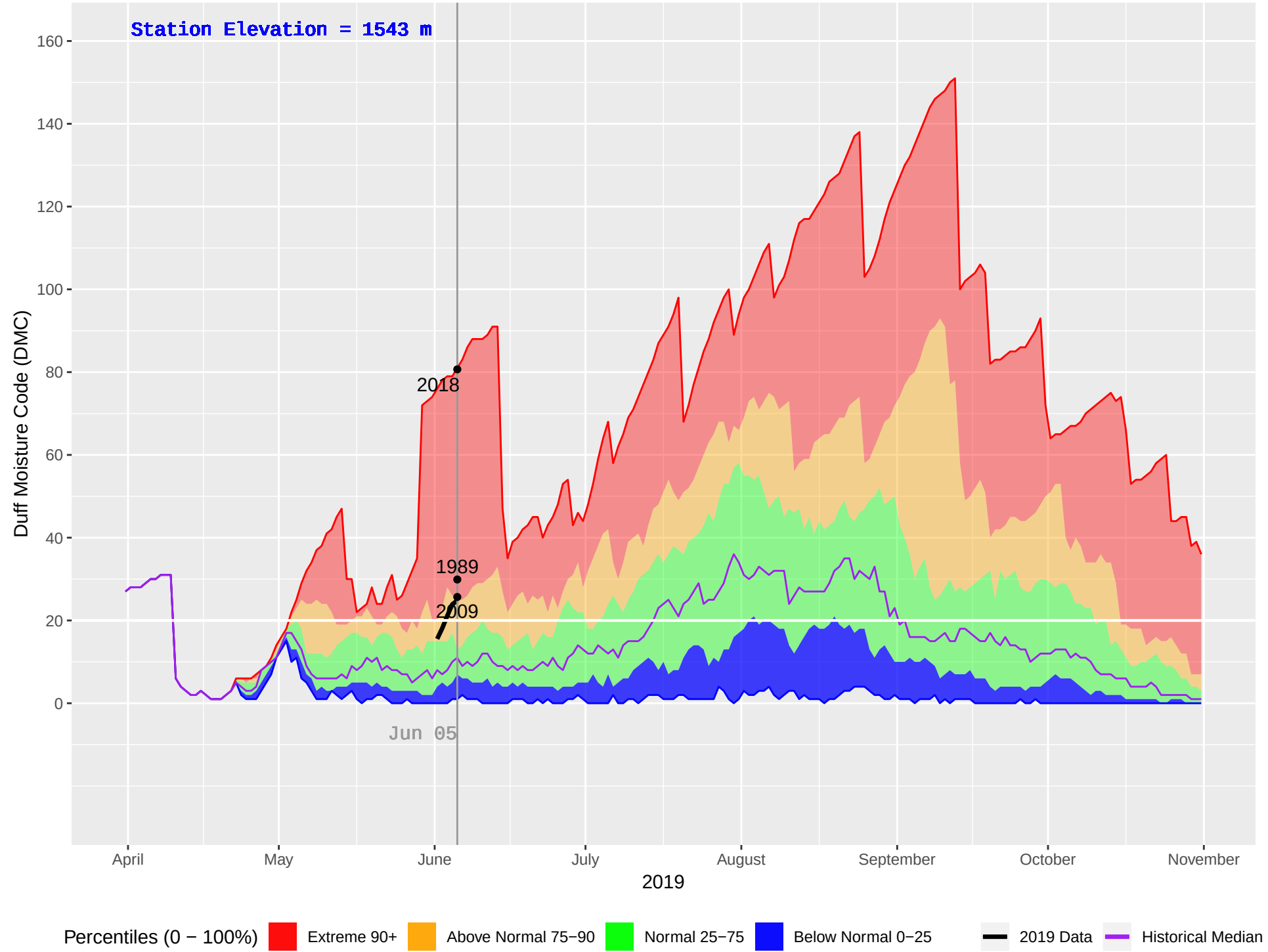
CAHILTY (253) : Historical (1987–2018), Current (2019) Daily Duff Moisture Code (DMC)
