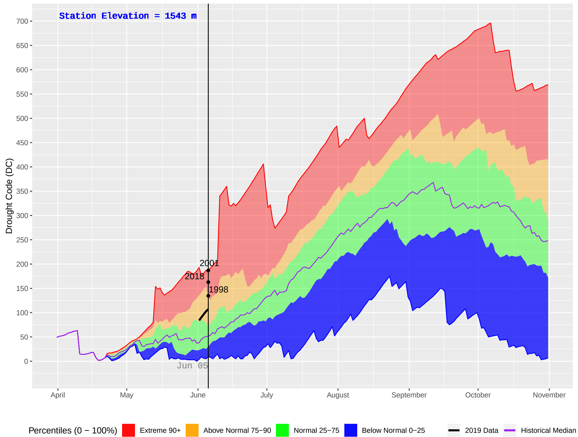
CAHILTY (253) : Historical (1987–2018) and Current (2019) Daily Drought Code (DC)
