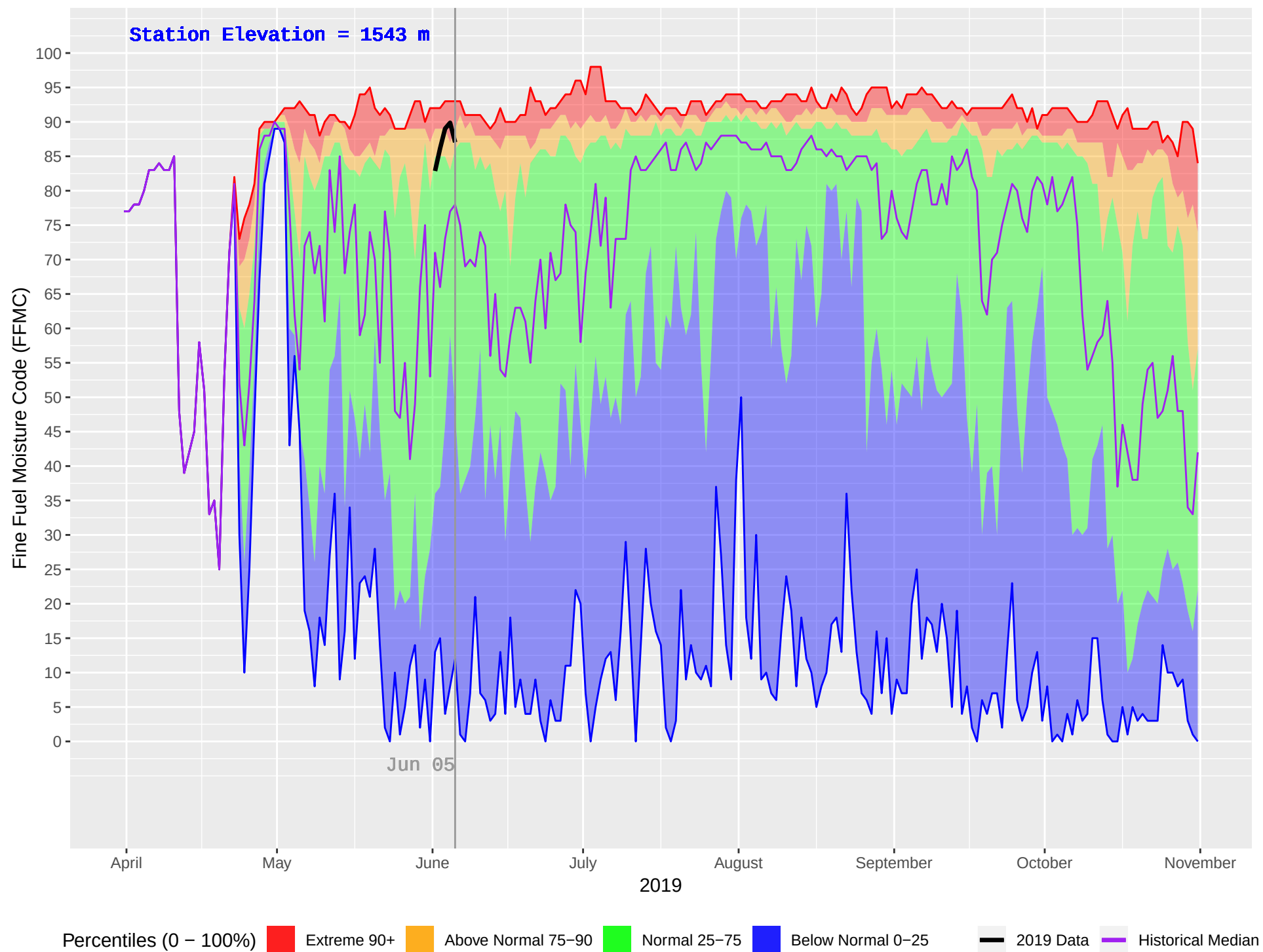
CAHILTY (253) : Historical (1987–2018) and Current (2019) Daily Fine Fuel Moisture Code (FFMC)
