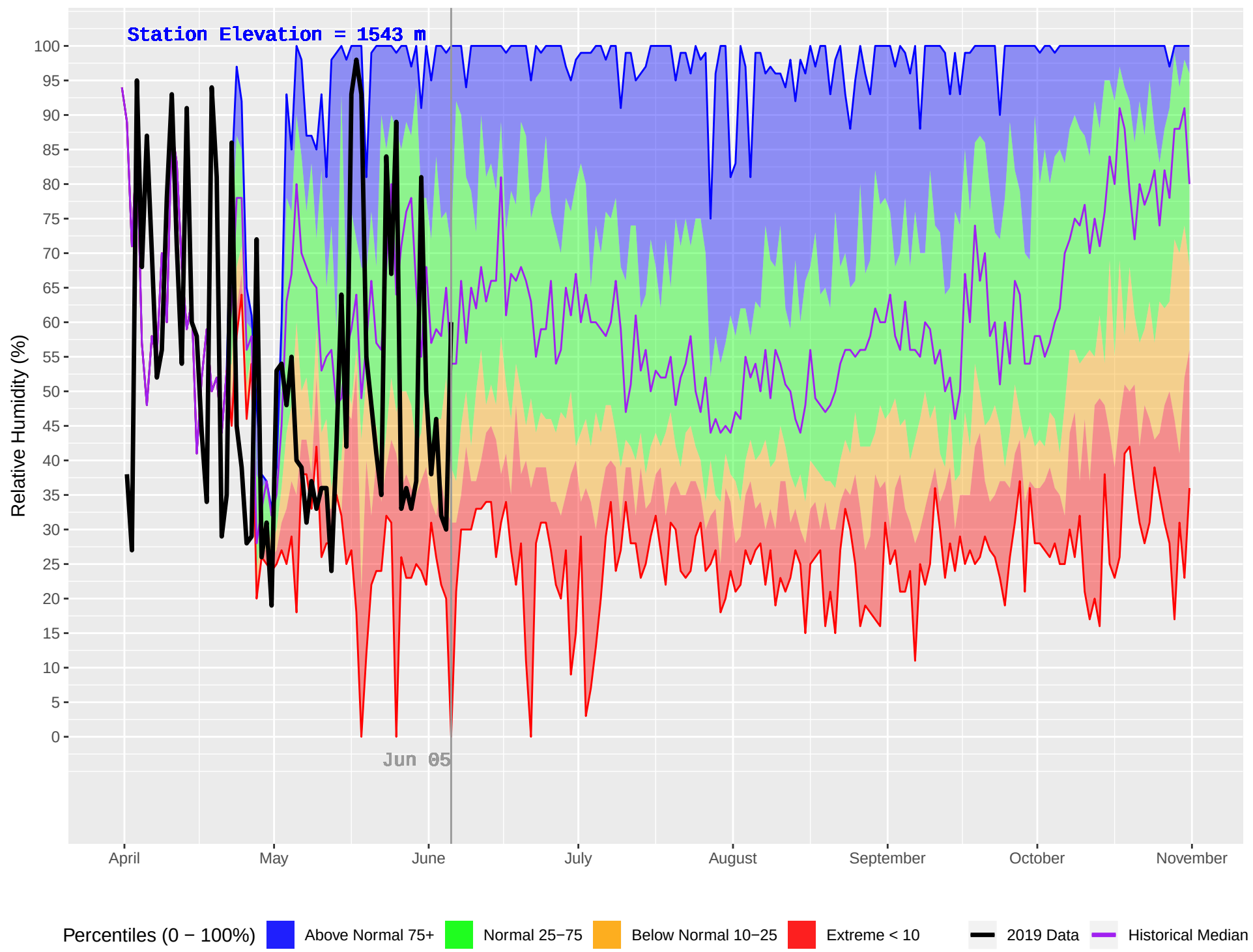
CAHILTY (253) : Historical (1987–2018) and Current (2019) Daily Relative Humidity
