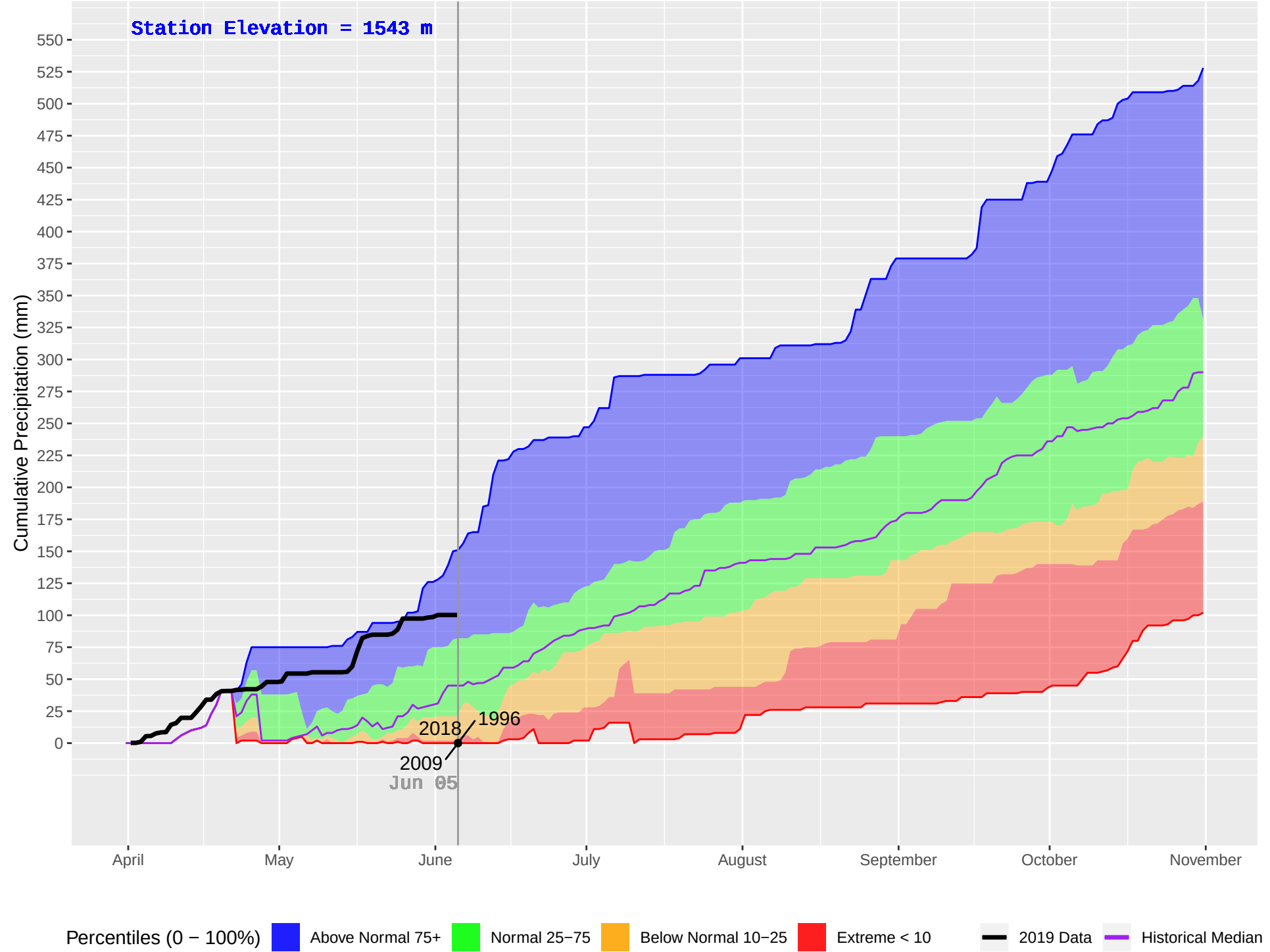
CAHILTY (253) : Historical (1987–2018), Current (2019) Daily Cumulative Precipitation
