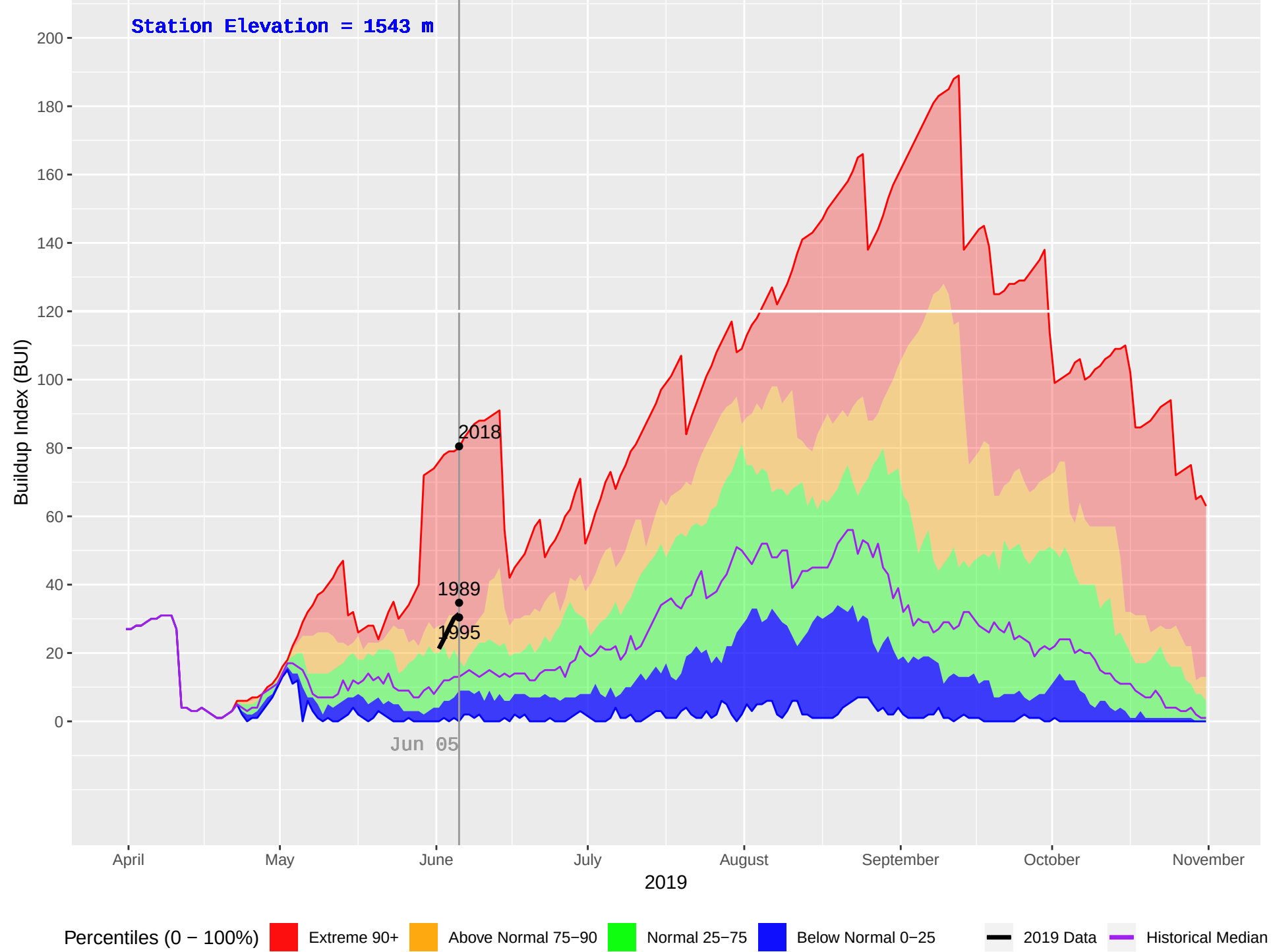
CAHILTY (253) : Historical (1987–2018), Current (2019) Daily Buildup Index (BUI)
